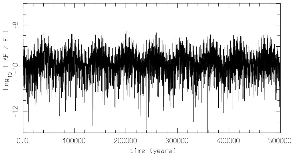
Figure 2. Check of our expansions of Hamiltonian (1).
