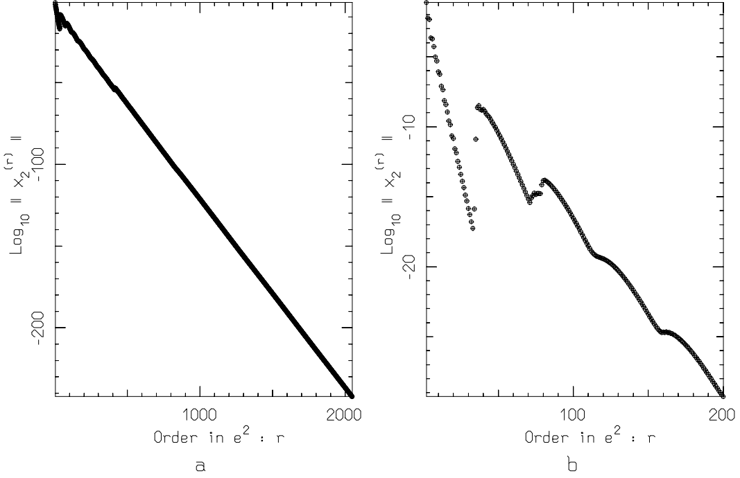
Figure 4. Decrease of the generating functions defined by the Kolmogorov's normalization algorithm. Figure 4a considers the construction of the invariant tori corresponding to the frequencies belonging to the set \Gamma'' defined in (51). The plotted values are the uniform upper bounds of the norms of \chi_2^{(r)} on the whole set \Gamma'' . Figure 4a has been enlarged in figure 4b, where we can appreciate the change of the slope occurring when the calculation of the norms is no more made starting by the coefficients of the expansions, but only iterating the estimates (i.e., for r = 33 ).
