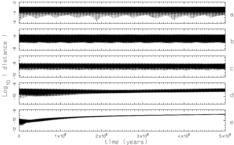
Figure 3. The distance d(t) between the numerically integrated orbit and the approximated motion (\tilde{\xi}_r(t), \tilde{\eta}_r(t)) calculated via the scheme (32). The curves a–e refer to the step r of Kolmogorov’s algorithm with r = 1, 5, 9, 11, 13 , respectively. The convergence may be appreciated by looking at the vertical scale. The drift effect in figure e is due to the error in the determination of the frequencies.
