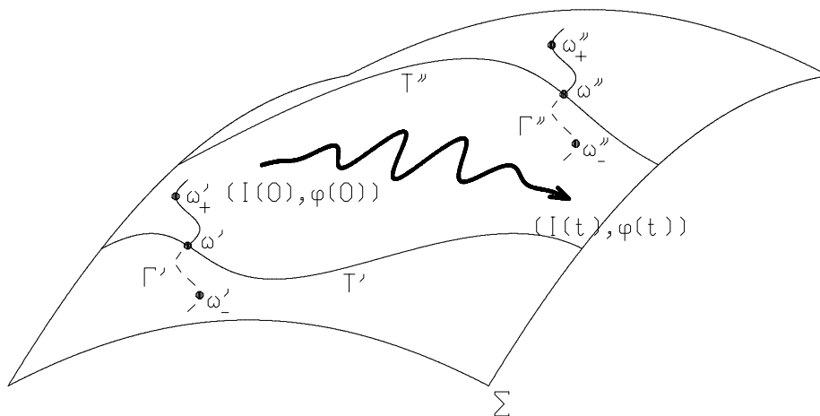
Figure 1. Illustrating the topological confinement of the orbit in the 4D phase space. The continuous curves \Gamma' and \Gamma'' represent two sets of 2D invariant tori that intersect transversally an energy surface. An orbit with initial datum in the gap between two tori will be eternally trapped in the same region (see text).
