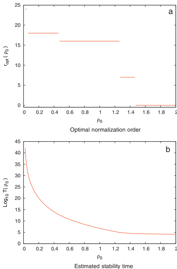
Fig. 1. Optimal normalization order r_{\text{opt}} and estimated stability time T(\varrho_0) evaluated according to the algorithm of Section 4.2. The time unit is the year. See text for more details.
